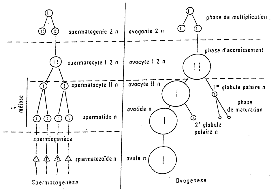
Comparaison spermatogenèse-ovogenese
